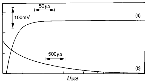
Fig. 1 (a) Formation and (b) decay of the transient in the flash photolysis of \text{trans}[\text{Co}(\text{en})_2(\text{OH}_2)(\text{SO}_3\text{-S})]^+ at 25 °C and pH 3.7
